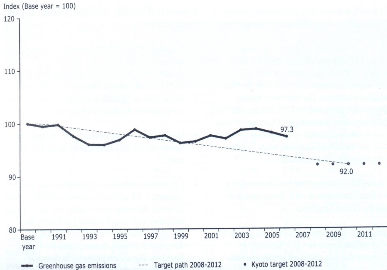
Figure ES.2 EU-15 GHG emissions 1990–2005 compared with target for 2008–2012 (excl. LULUCF)
